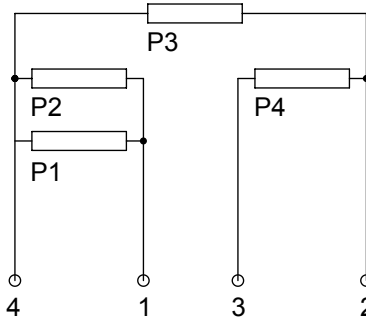
wiring diagram
